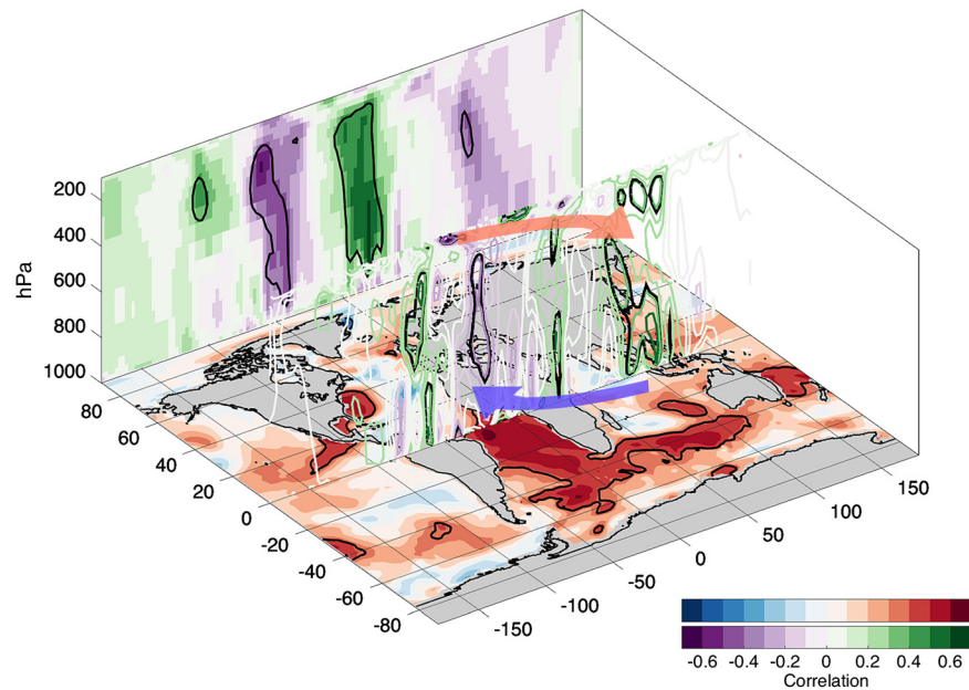
Fig. 4. Atmosphere-ocean response to solar forcing. TM-17 \delta^{18}\text{O} correlations with ensemble mean CSM-LME solar forcing only SST anomalies ( x/y plane shading), omega ( \omega ) ( x/z contours), and the zonal mass streamfunction ( \psi ) ( x/z shading) averaged 5^\circ\text{S} – 5^\circ\text{N} . The sign convention is such that positive (negative) \omega and \psi correlations correspond to subsidence (convection) and clockwise (counter-clockwise) circulations, respectively. Note the \psi section on the back wall corresponds to values straddling the equator. Thick black contours indicate correlation significance at 95% confidence level. The blue arrow illustrates surface flow converging onto the warm tropical Atlantic, whereas the red arrow indicates upper-level divergence associated with the resulting deep convection.
