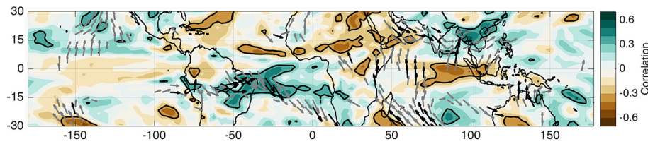
Fig. 5. TM-17 \delta^{18}\text{O} correlated with ensemble mean CSM-LME solar forcing-only precipitation. TM-17 \delta^{18}\text{O} correlated with CSM-LME total precipitation rate (shading) and 850 mb wind fields (arrows). Thick black contours and black (grey) arrows indicate correlation significance at 95% (80%) confidence level based on the distribution of 1,000 randomly generated low-pass filtered time series. All time series were subjected to a 50-year low pass filter.
