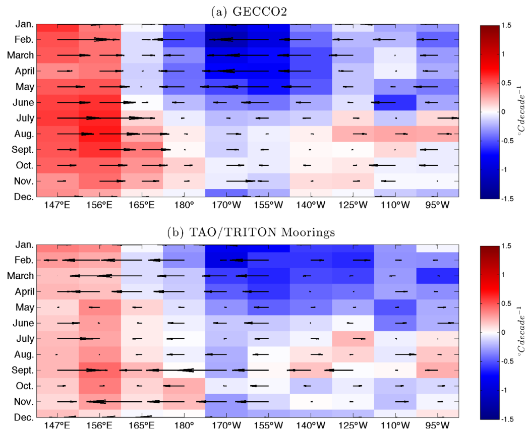
Figure 12. Same as Figure 7a, but for GECCO2 SST and zonal wind stress trends (a) and TAO/TRITON SST and zonal wind stress trends (b). All moorings from 5°S to 5°N were averaged along each longitude line. The maximum zonal wind stress vector represents 0.91 N m -2 decade -1 and 0.02 N m -2 decade -1 for Figures 12a and 12b, respectively.
