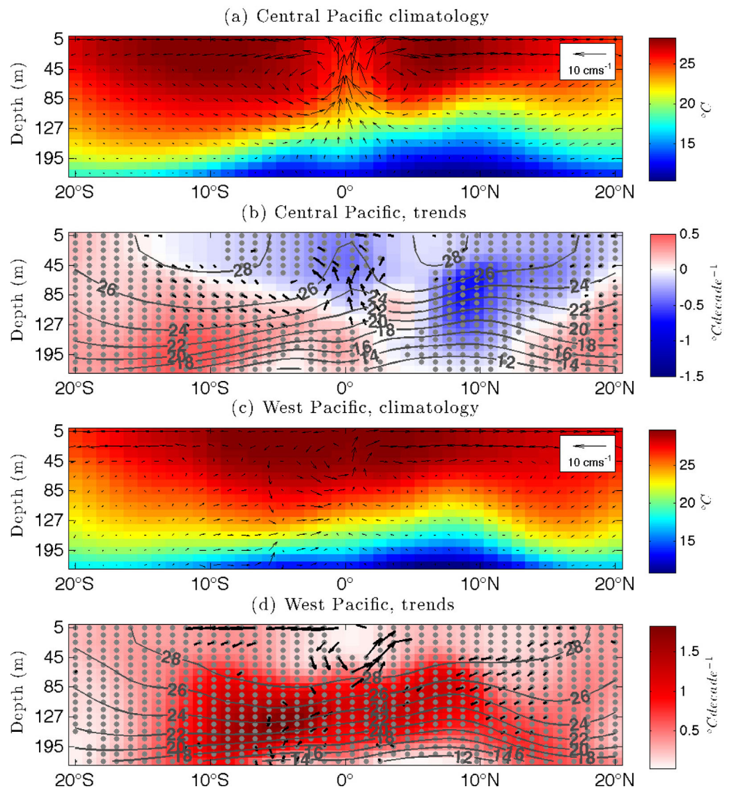
Figure 6. Same as Figure 5, but a latitude/depth cross sections of temperature and currents. Averaged from 180° to 120°W (a, b) and 140°E to 180° (c, d). Gray contours in Figures 6b and 6d represent the mean climatology of temperature for the respective region. Stippling and vectors represent significance at the 95% level. The maximum current trend vector represents 2.5 cm s -1 decade -1 and 3.2 cm s -1 decade -1 for Figures 6b and 6d, respectively.
