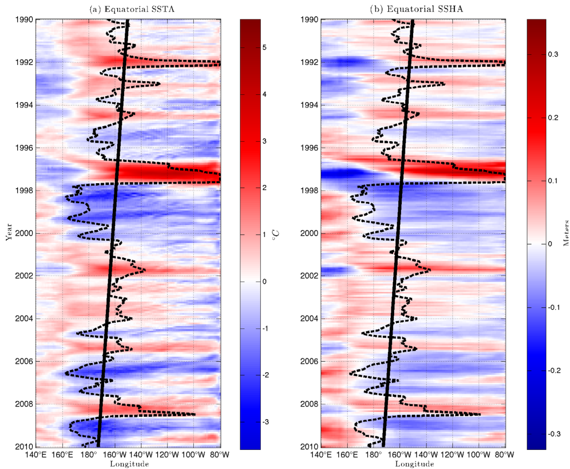
Figure 3. Time/longitude plots of SST anomalies (a) and SSH anomalies (b) averaged over 5°S–5°N. The dashed lines outline the 27.5°C isotherm. The line of best fit is in solid black.
