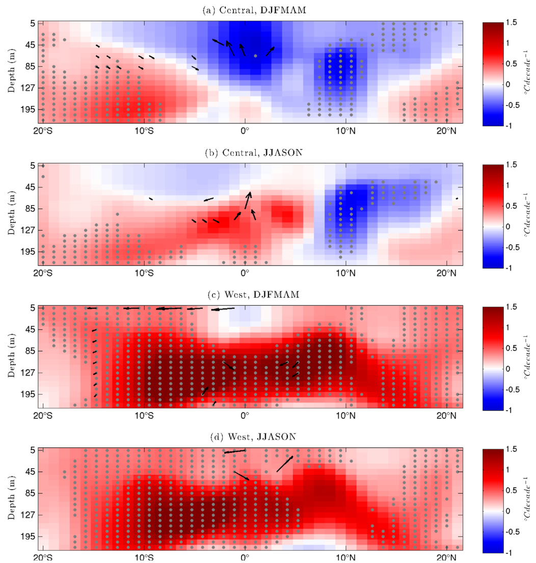
Figure 10. Same as Figures 6b and 6d, but averaged over DJFMAM (a) and JJASON (b). The maximum current trend vector represents 2.96, 3.2, 2.8, and 3.5 \text{cm s}^{-1} \text{decade}^{-1} for Figures 10a–10d, respectively.
