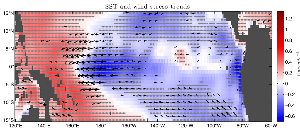
Figure 2. Trends in SST ( ^{\circ}\text{C decade}^{-1} ) and surface wind stress ( \text{N m}^{-2} \text{ decade}^{-1} ) during 1990–2009. Stippling indicates SST trend significance at the 95% level. Wind stress vectors are only plotted where significant at the 95% level. The maximum wind stress trend vector represents 0.02 \text{ N m}^{-2} \text{ decade}^{-1} .
