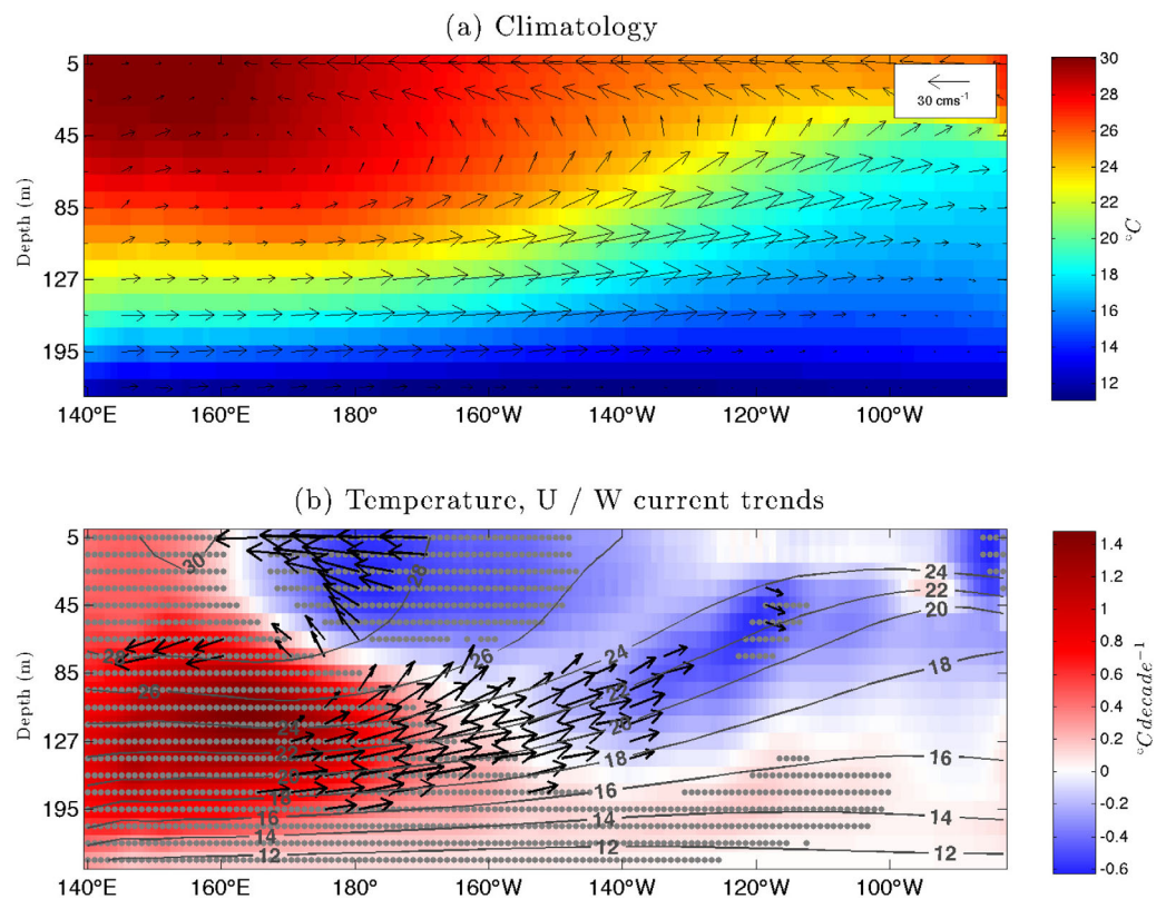
Figure 5. Longitude/depth cross sections of temperature (shading) and currents (vectors) averaged over 2.5°S–2.5°N for (a) mean climatology (1980–2010) and the linear trends during 1990–2009 (b). Temperature trends ( ^{\circ}\text{C decade}^{-1} ) are in shading and U / W current trends ( \text{cm s}^{-1} \text{ decade}^{-1} ) are black vectors. Gray contours in (b) represent the mean climatology of temperature. Stippling indicates temperature trend significance at the 95% level. Current vectors are only plotted where significant at the 95% level. The maximum current trend vector represents 8.5 \text{ cm s}^{-1} \text{ decade}^{-1} . Note: in the figure, the vertical velocity component of current vectors has been scaled by 10^4 .
