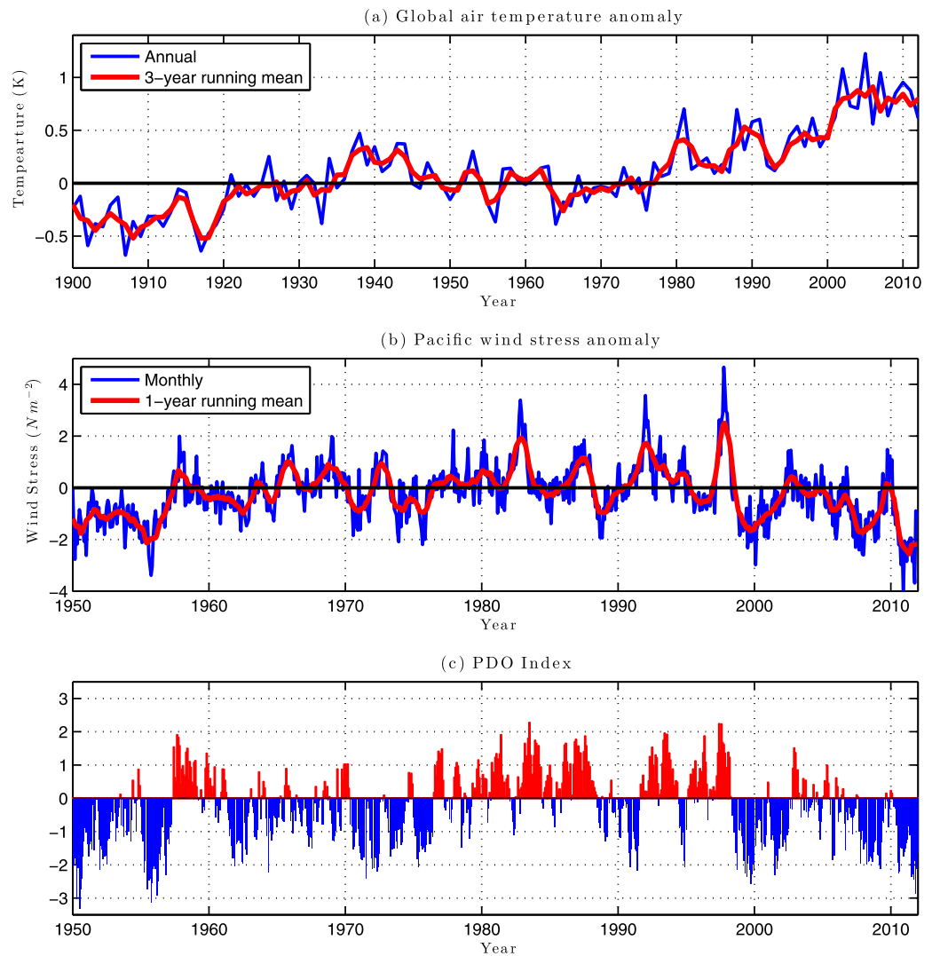
Figure 1. GISS global-averaged surface air temperature anomalies (a), zonal wind stress anomalies averaged 5°S–5°N, 180°–150°W (b), and the Pacific Decadal Oscillation (PDO) Index (c). (top) From January 1900 to December 2011, while both (b) and (c) from January 1948 to December 2011. Blue time series are annual (Figure 1a), monthly (Figure 1b), and negative (Figure 1c) data. Red time series are 3 (Figure 1a) and 1 year (Figure 1b) running means and positive PDO values (Figure 1c). Wind stress anomalies were scaled by 100.
