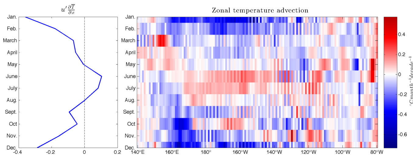
Figure 8. Same as Figure 7, but zonal surface temperature advection trends ( ^{\circ}\text{C month}^{-1} \text{ decade}^{-1} ) from 1990 to 2009. Zonal temperature advection trends averaged from 160^{\circ}\text{E} to 150^{\circ}\text{W} are shown to the left. This data were taken from the raw model grid.
