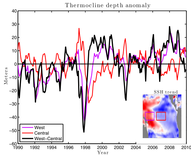
Figure 4. Time series for the depth of the 20°C isotherm averaged from 5°S–5°N, 140°E–180°W (purple box/line), 5°S–5°N, and 170°W–130°W (red box/line). The difference of the red box from the purple box is shown in black. Positive (negative) anomalies represent a deeper (shallower) thermocline. The insert shows the SSH trend.
