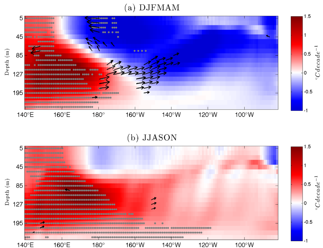
Figure 9. Same as Figure 5b, but linear trends of DJFMAM (a) and JJASON (b) from 1990 to 2009. The maximum current trend vector represents 16.1 \text{ cm s}^{-1} \text{ decade}^{-1} and 5.3 \text{ cm s}^{-1} \text{ decade}^{-1} for Figures 9a and 9b, respectively.
