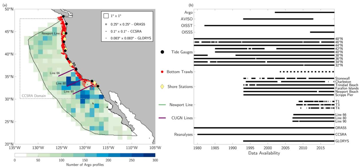
Fig. 1. (a) Spatial distribution and (b) temporal availability of all data sets used in this study. Shading in (a) denotes total number of Argo profiles since 2002, binned in 1^\circ \times 1^\circ grid cells. Black line outlines in the CCLME. Dashed gray line denotes the CCSRA regional domain. Black lines for each dataset in (b) indicates that the data was available for the given time step somewhere within the CCLME.
