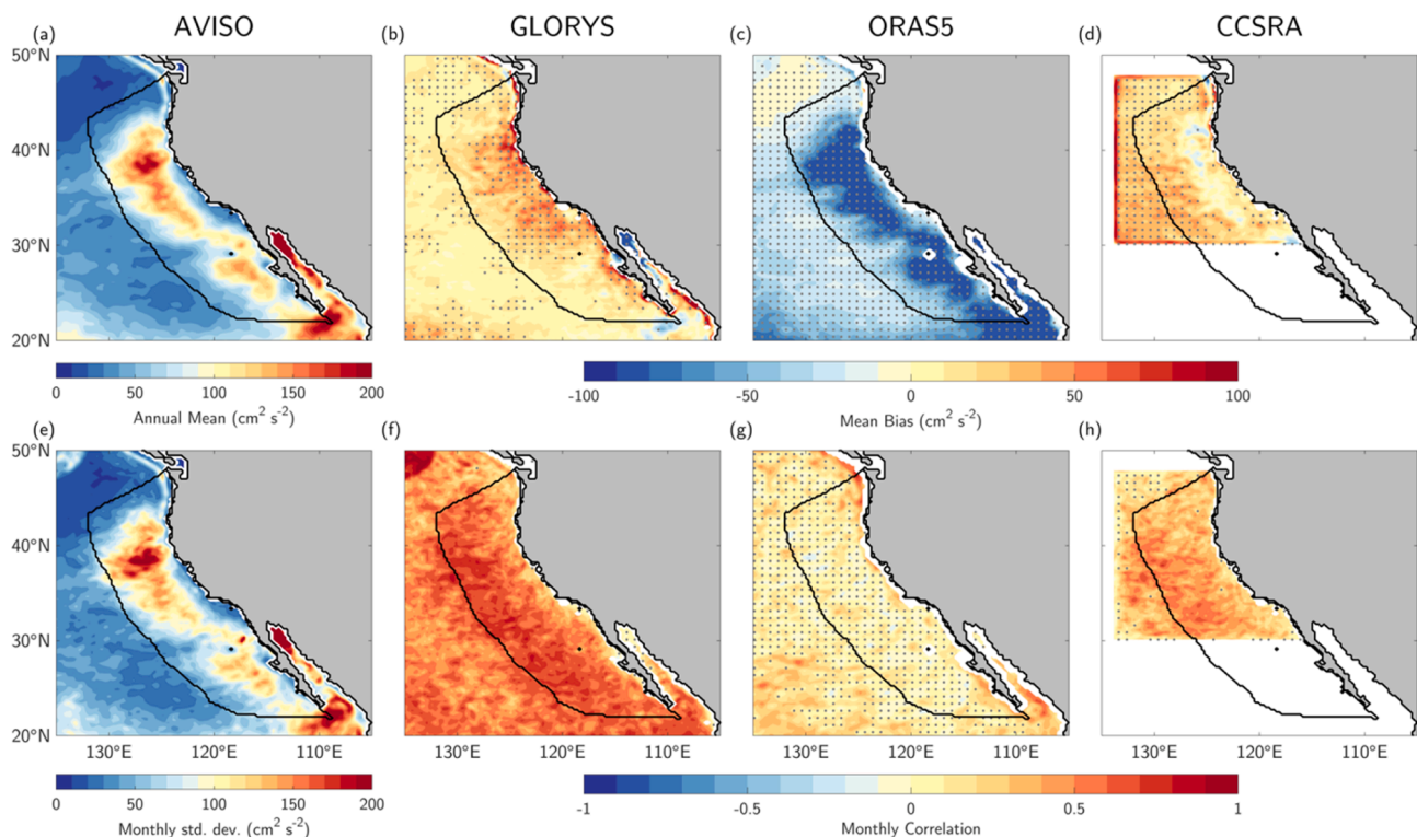
Fig. 15. (a) Annual mean geostrophic Eddy Kinetic Energy (EKE; \text{cm}^2 \text{s}^{-2} ) based on SSH anomalies from AVISO satellite observations. (b)–(d) Annual mean EKE biases in GLORYS, ORAS5, and CCSRA, respectively. (e) Monthly mean EKE standard deviation in AVISO. (f)–(h) Anomaly correlation coefficients between monthly mean EKE values from AVISO and each reanalysis. Stipples in (b)–(d) indicate a significant mean bias with 95% confidence. Stipples in (f)–(h) indicate an insignificant correlation with 95% confidence.
