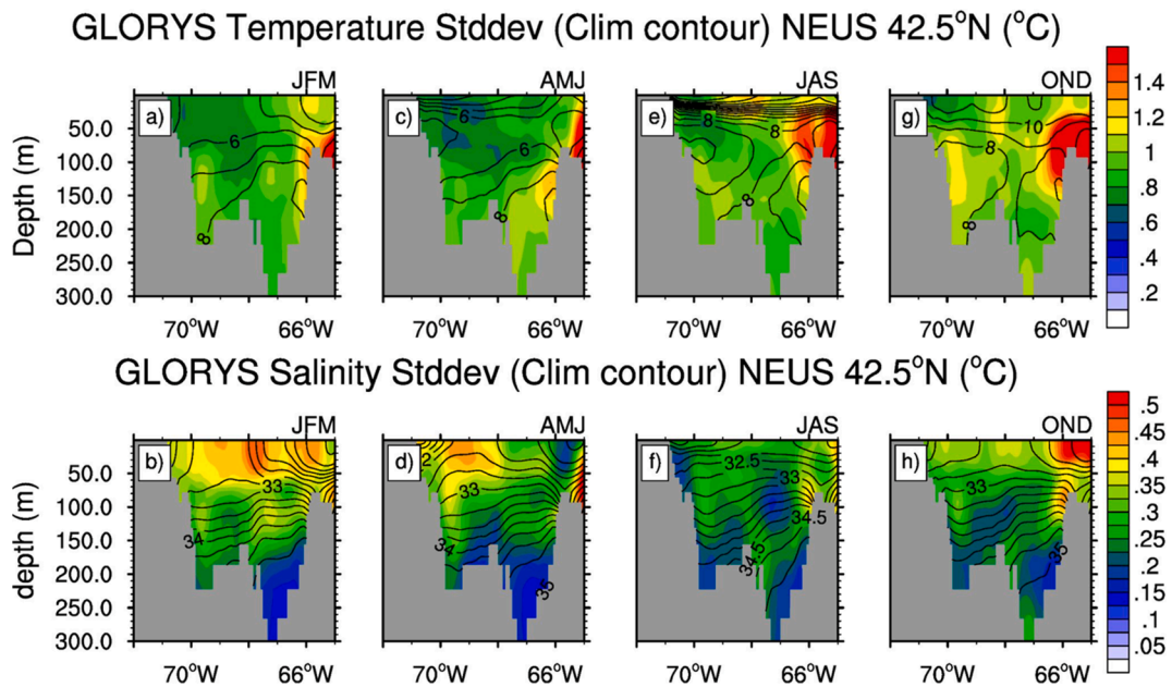
Fig. 17. Vertical cross-sections of (a,c,e,g) temperature ( ^{\circ}\text{C} ) and (b,d,f,h) salinity (psu) standard deviation (shading) and climatology (contours) along 42.5^{\circ}\text{N} in the NEUS for (a,b) JFM, (c,d) AMJ, (e,f) JAS and (g,h) OND. Location of the cross section is shown as a gray line in Fig. 1.
