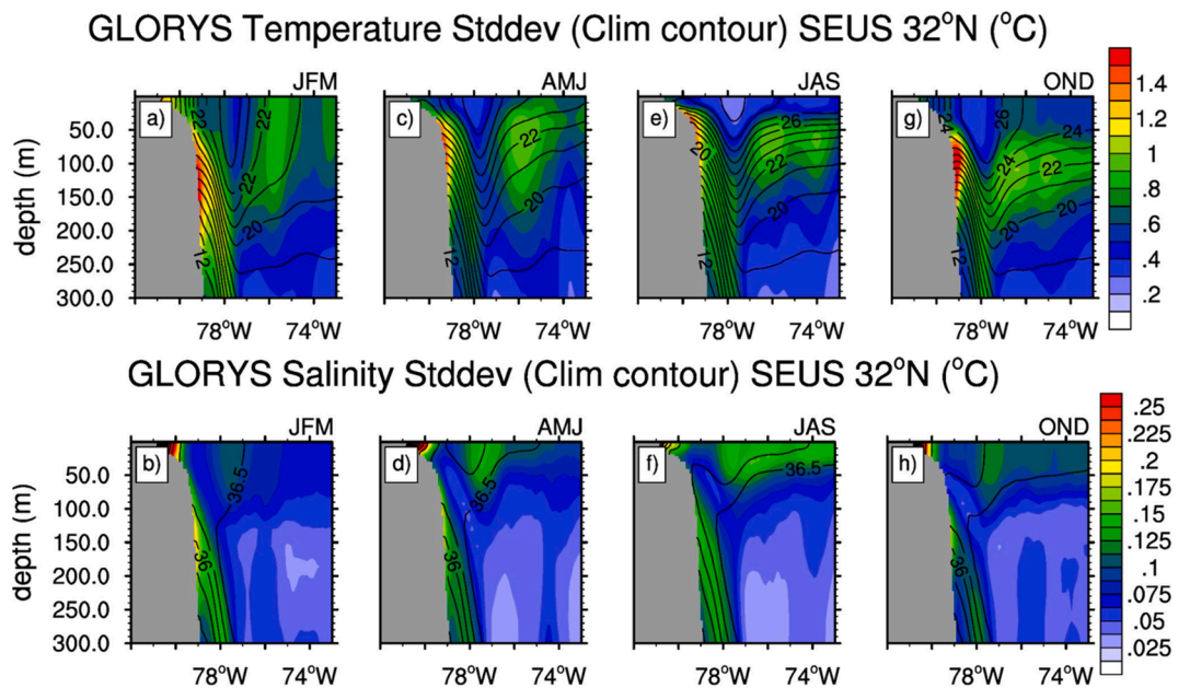
Fig. 18. As in Fig. 17 but for vertical cross-sections of temperature and salinity along 32^{\circ}\text{N} in the SEUS.
