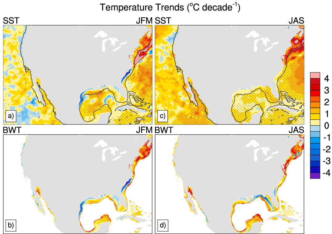
Fig. 15. Linear trends (f1993–2019) in (a,c) SST, and (b,d) BWT for (left) JFM and (right) JAS. The 400 m isobath (black line) is shown in (a,c). Significant trends (95%) using Mann-Kendall non-parametric test are indicated by stippling.
